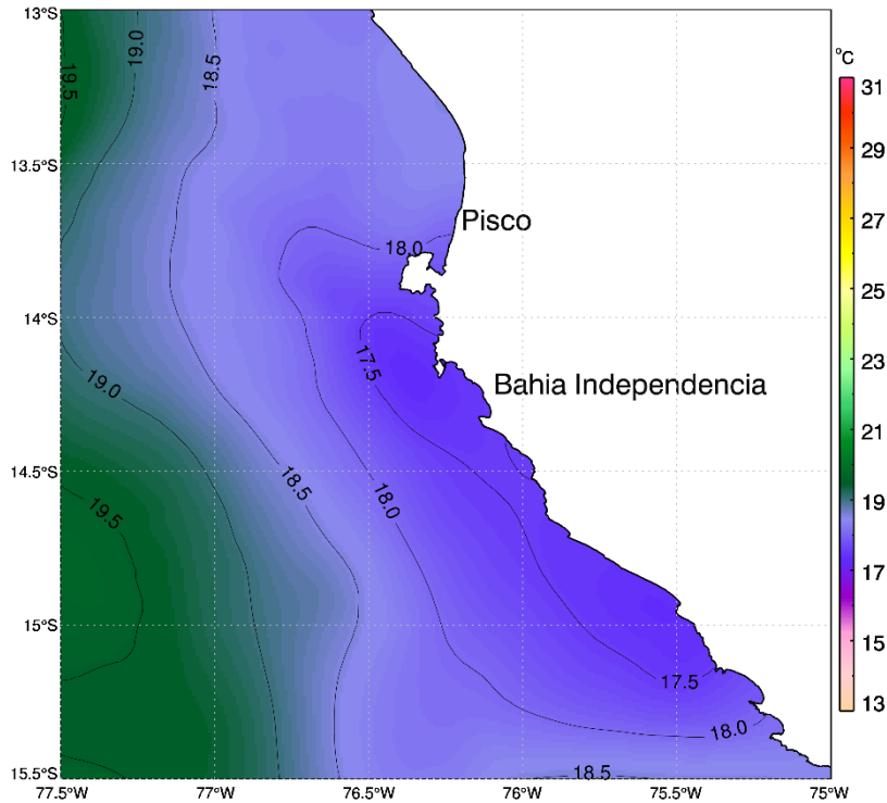
Temperatura Superficial de Mar (TSM) 13°00'S – 15°00'S
